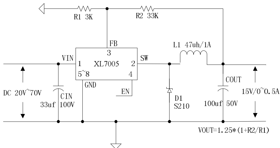
Figure5. XL7005 System Application (VIN=20V~70V, VOUT=15V)
