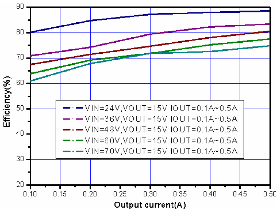
Figure6. XL7005 System Application (Efficiency VS Output Current)
